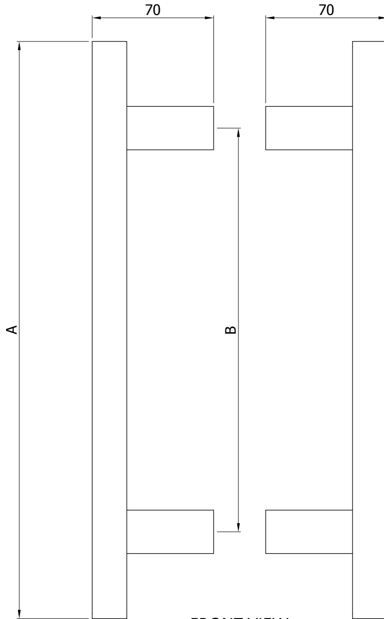
FRONT VIEW
