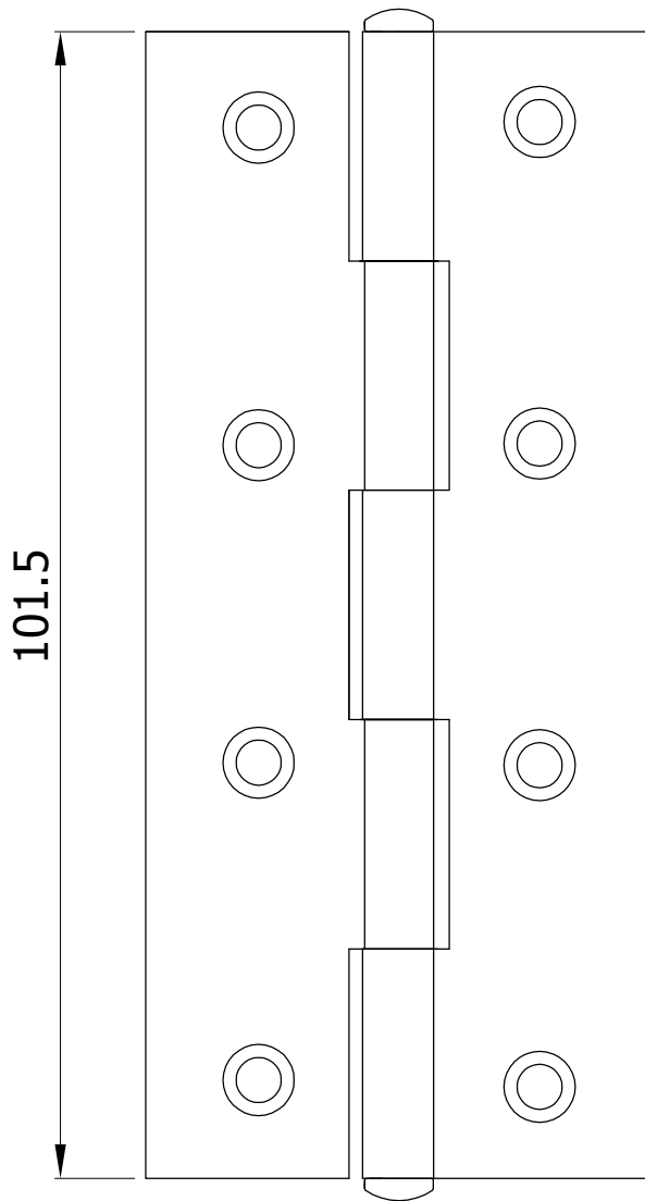
FRONT VIEW
